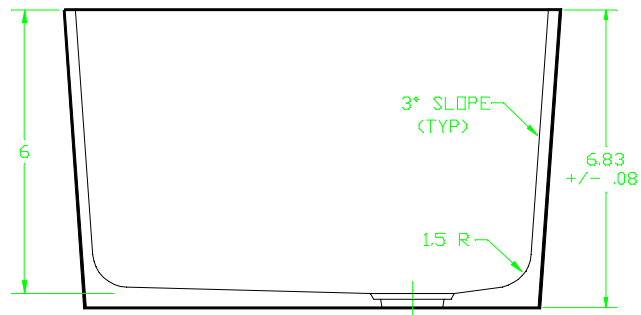
FRONT VIEW
