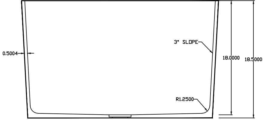
SECTION VIEW
